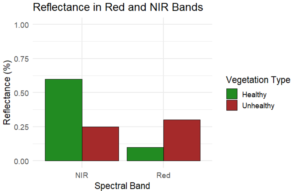
Figure 2 – Reflectance in the red and NIR bands for healthy and unhealthy vegetation.
