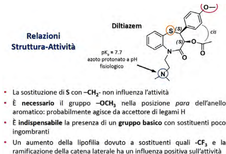
Figura 25 - Benzotiazepine
